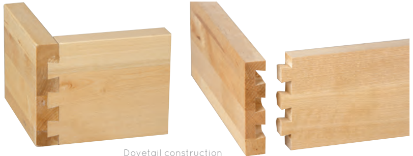
Dovetail construction
