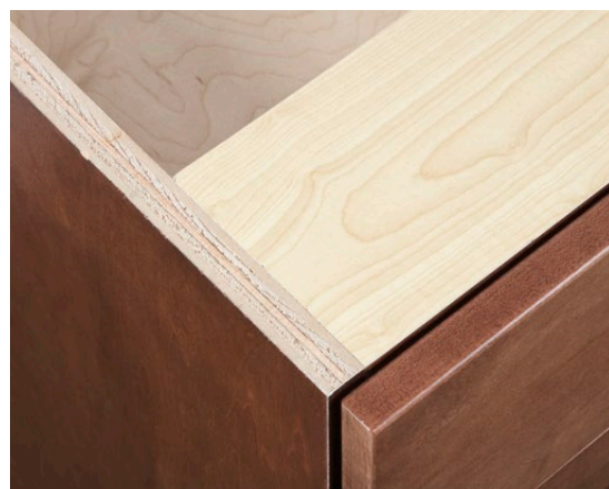
▲ 5/8" THICK PLYWOOD end panels Shown with finished end.
